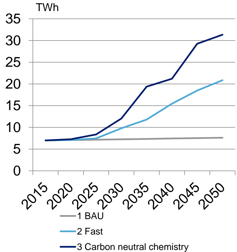
Electricity demand
