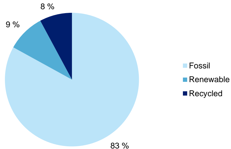
2050 outcome
